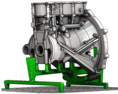
11(a) Stabilizing bars at either end of the casting
