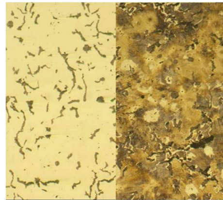
13(b) 8% Nodularity and 94% pearlite
