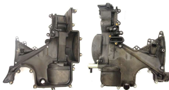
Figure 8. Inner and outer surfaces of the left-side plastic casings at the conclusion of the 100-hour engine test.
