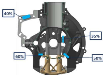
15(a) Nodularity in the 2.7 mm nominal outer walls
