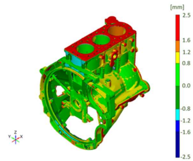
10(a) Cylinder block – top
