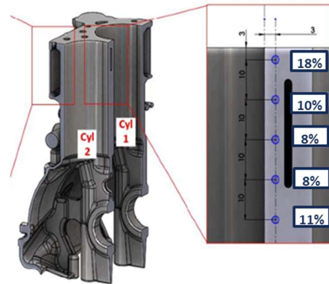
13(a) Nodularity as a function of bore height
