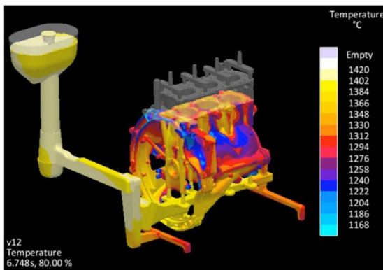
9(b) Temperature profile simulation
