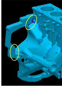
11(b) Residual stress concentration in original design
