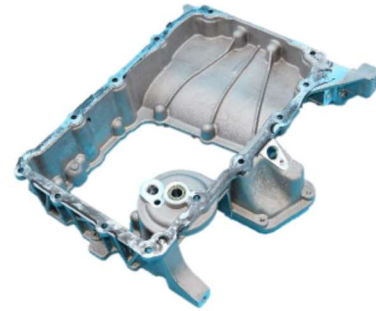
1(b) Upper oil pan (3.45 kg)
