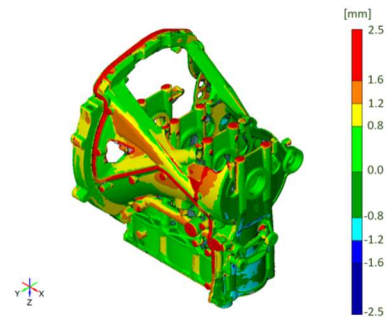
10(b) Cylinder block – bottom
