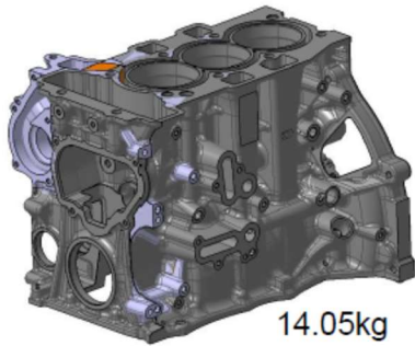
Figure 5. The removal of the integrated water pump housing and five bosses in the 48-Volt configuration reduces the aluminum cylinder block weight from 14.05 kg to 13.46 kg, resulting in a reduction of the assembled block weight from 21.06 to 20.47 kg including the bearing caps, upper and lower oil pan and fasteners.
