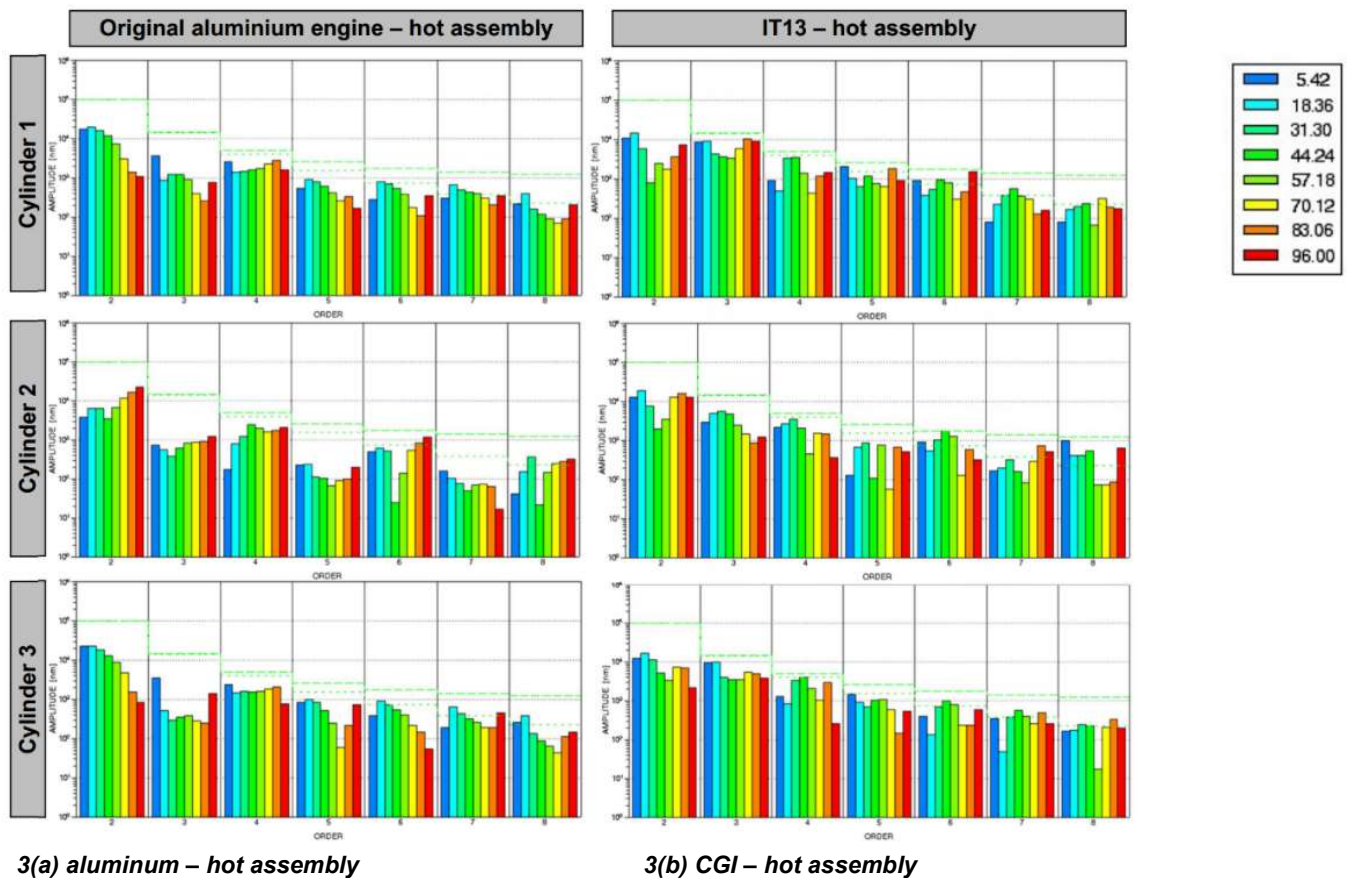
Figure 3. Cylinder bore distortion in the original aluminum engine and in the CGI engine; both concepts satisfy piston ring conformability with 1 \mu\text{m} oil film (nm).
