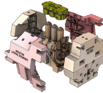
12(a) Exploded view of the cylinder block core package
