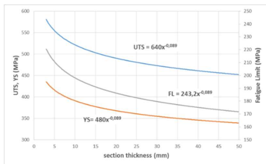
15(b) Design properties as a function of wall thickness
