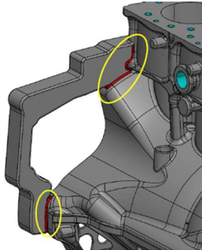
11(c) Increased fillet radii to minimize residual stress
