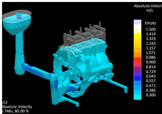
9(a) Metal flow velocity simulation
